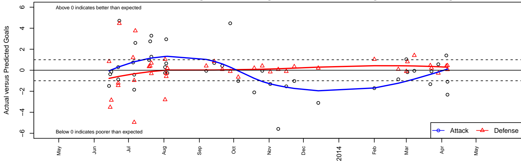
NORTAC Comets G01 Dots are actual minus expected GF (blue circles) and GA (red triangles). Blue line is smoothed change in attack strength. Red is smoothed change in defense strength.
